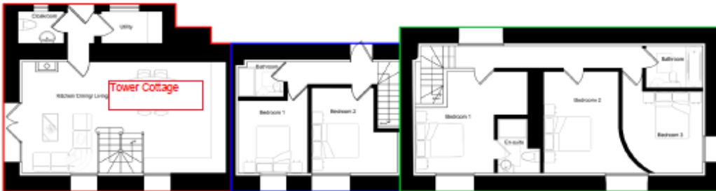
Proposed First Floor 1:100
